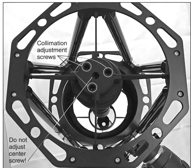
Figure 8. Secondary mirror collimation is done by adjusting the three socket head capscrews on the front of the telescope.
