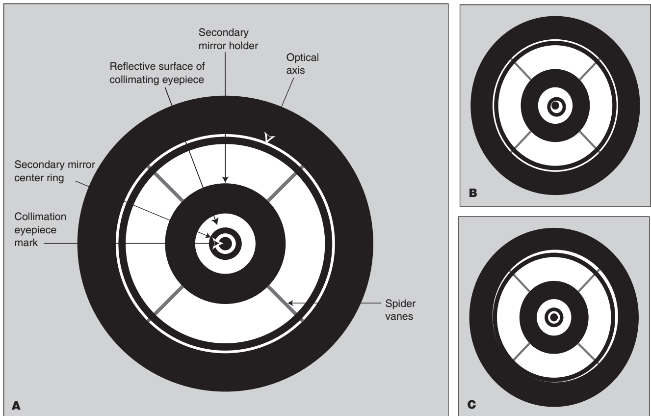
Figure 9. The view through a collimating eyepiece (not to scale). A) Shows the Ritchey-Chretien aligned with all components identified. B) Shows the secondary out of alignment. C) Shows the optical axis out of alignment.
